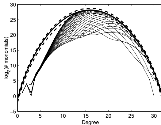
Figure 2: The number of monomials of each degree in each of the 32 Boolean functions of the g -function. The thick solid line and the two dashed lines denote the average and variance for an ideal random function.
